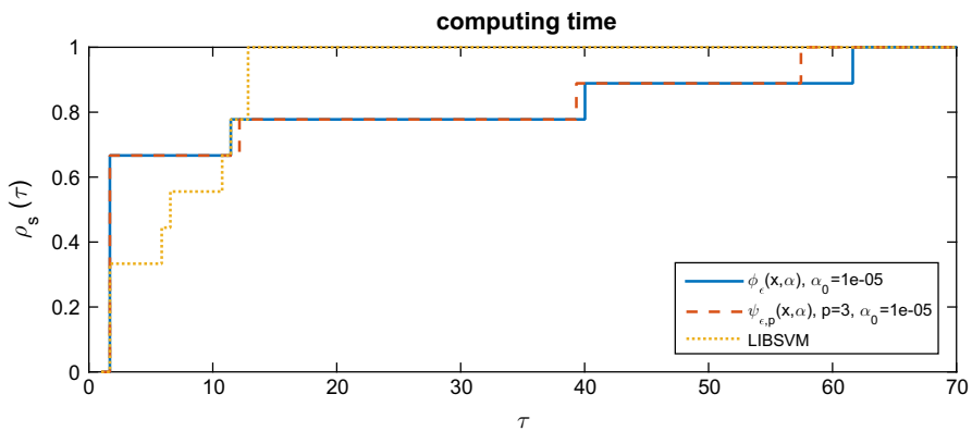
Fig. 8 Performance profile of \phi_\varepsilon(x, \alpha) , \psi_{\varepsilon,p}(x, \alpha) with p = 3 and LIBSVM
