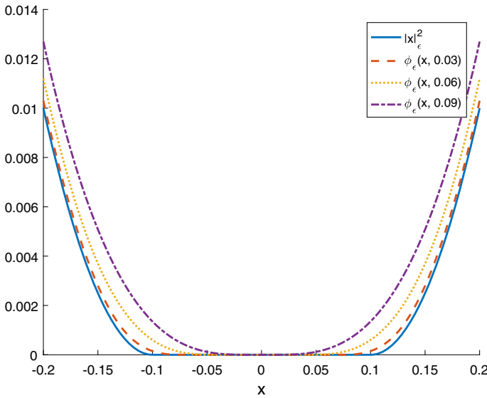
Fig. 1 Graphs of \phi_\varepsilon(x, \alpha) with \varepsilon = 0.1 and \alpha = 0.03, 0.06, 0.09
