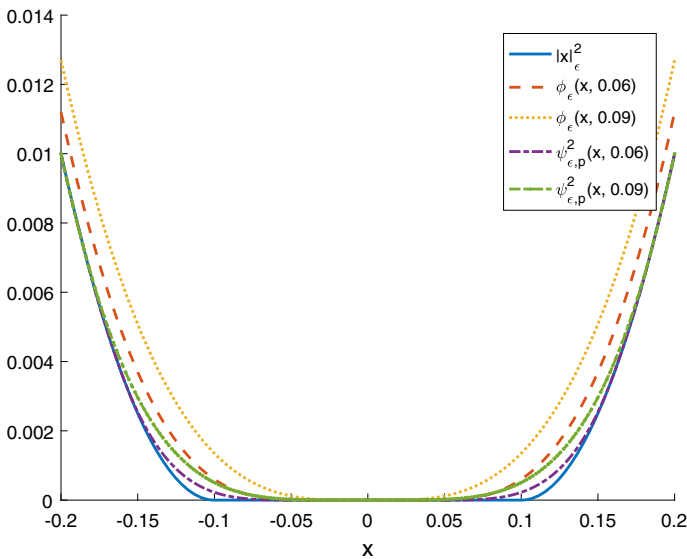
Fig. 3 Graphs of |x|_{\epsilon}^2, \phi_{\epsilon}(x, \alpha) and \psi_{\epsilon,p}^2(x, \alpha) with \epsilon = 0.1, \alpha = 0.06, 0.09 and p = 2
