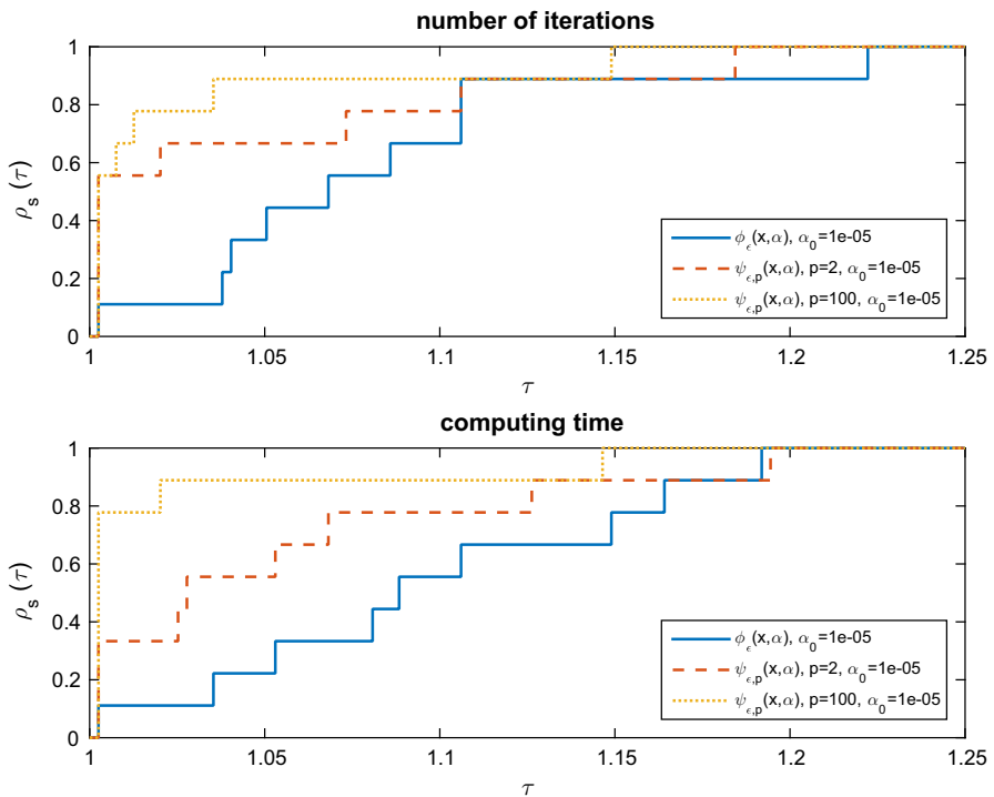
Fig. 7 Performance profile of \phi_\varepsilon(x, \alpha) and \psi_{\varepsilon,p}(x, \alpha) with p = 2, 100
