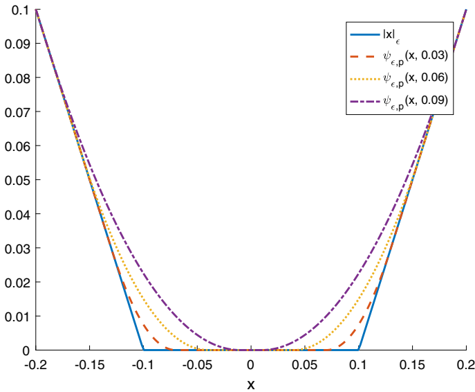
Fig. 2 Graphs of \psi_{\epsilon,p}(x, \alpha) with \epsilon = 0.1, \alpha = 0.03, 0.06, 0.09 and p = 2
