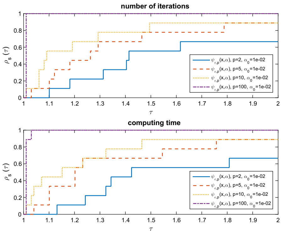
Fig. 6 Performance profile of \psi_{\varepsilon,p}(x, \alpha) when p = 2, 5, 10, 100
