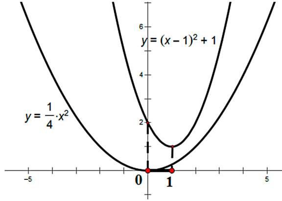
Figure 1. Illustration of Example 3.1.
